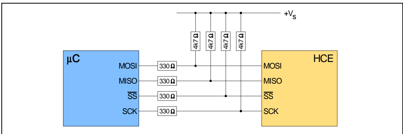
Fig. 7: SPI bus application circuit for Sensortechinics' HCE pressure sensors
